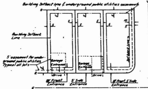
TYPICAL LOTS SHOWING SETBACK LINES AND PUBLIC UTILITIES EASEMENTS
